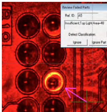
Solder Fillet Quality Inspection
